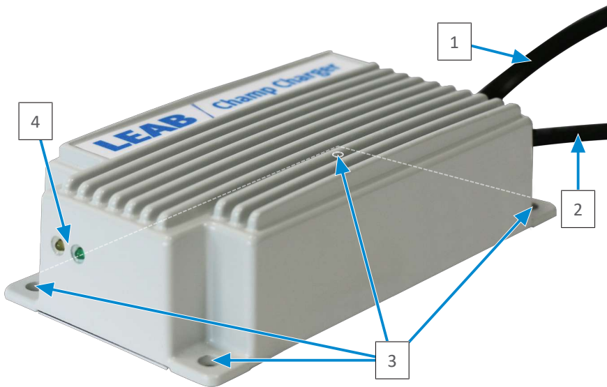
Fig. 1: Champ charger
